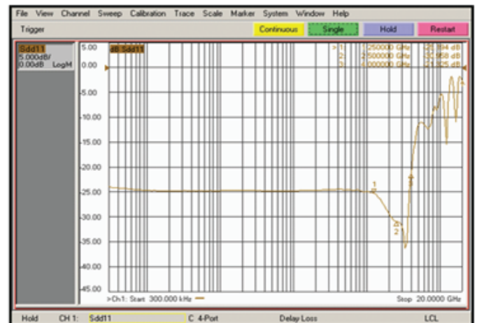
Fig.2 Return Loss
