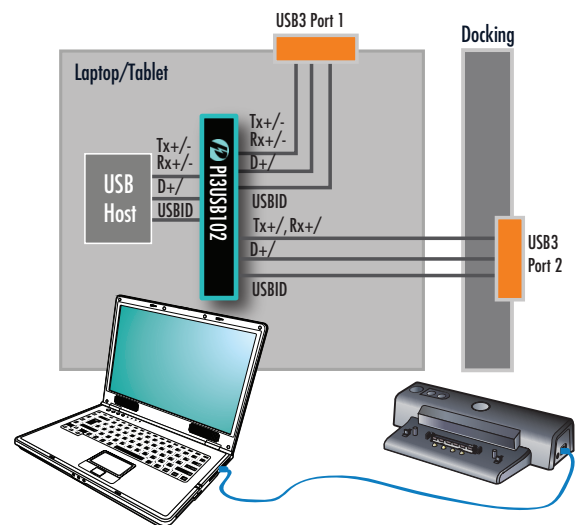
Fig 5. USB 3.0 Switch in a Notebook Docking Application
