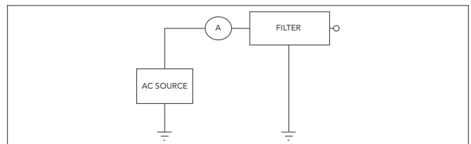
Figure 4. Leakage Current Test Circuit.
