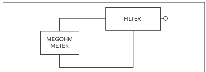
Figure 7. Setup for Insulation Resistance Test.
