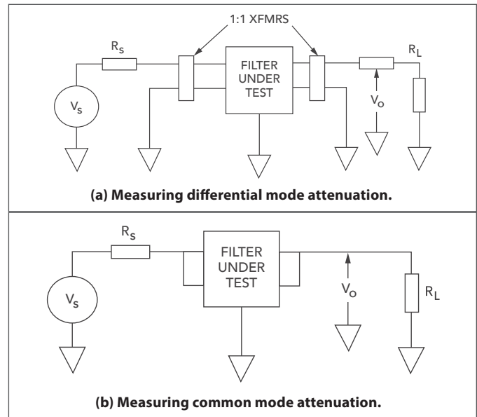
Figure 1. A Typical Test Setup for Measuring Filter Attenuation.
