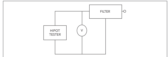
Figure 6. Typical Test Setup for Dielectric Withstand or Hi-Pot.
