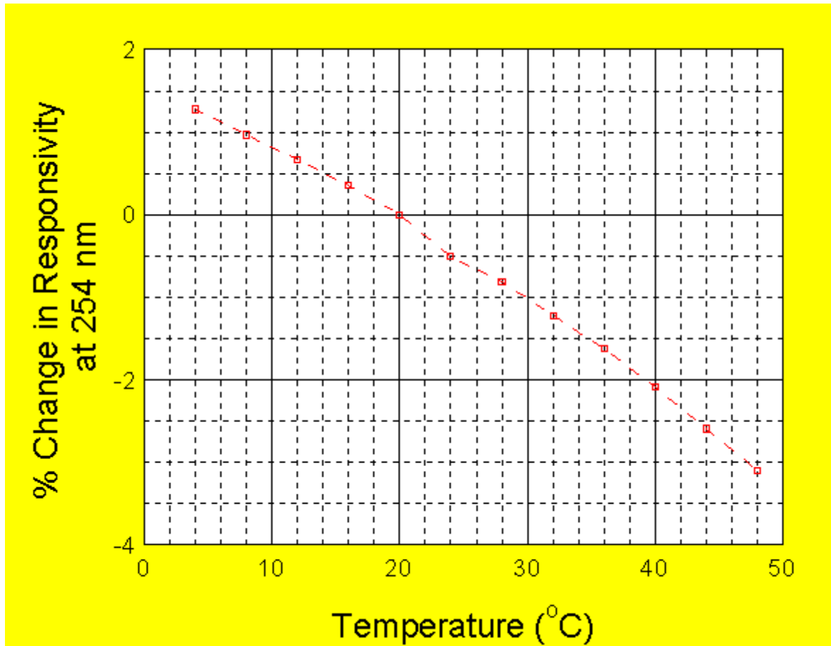
Fig. 3: Change in 254 nm responsivity of SXUV series diodes with temperature
