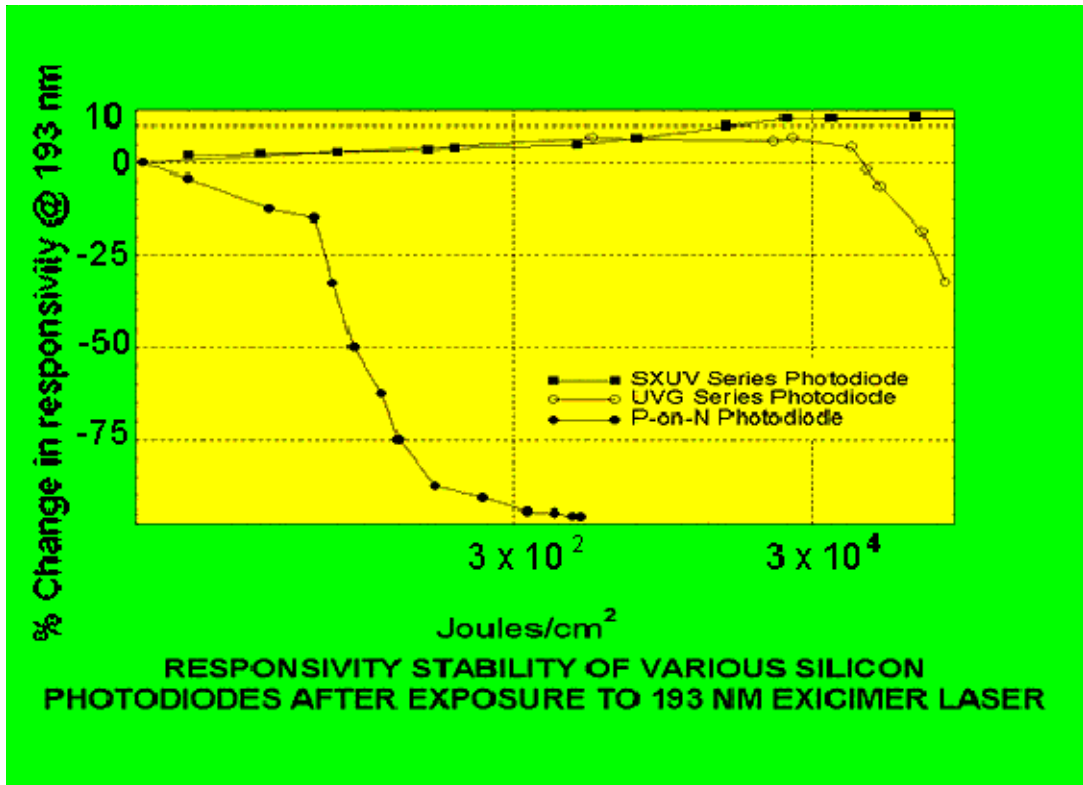
Fig. 1: Stability of SXUV diodes compared to UVG series and p-on-n diodes when exposed to 193nm radiation
