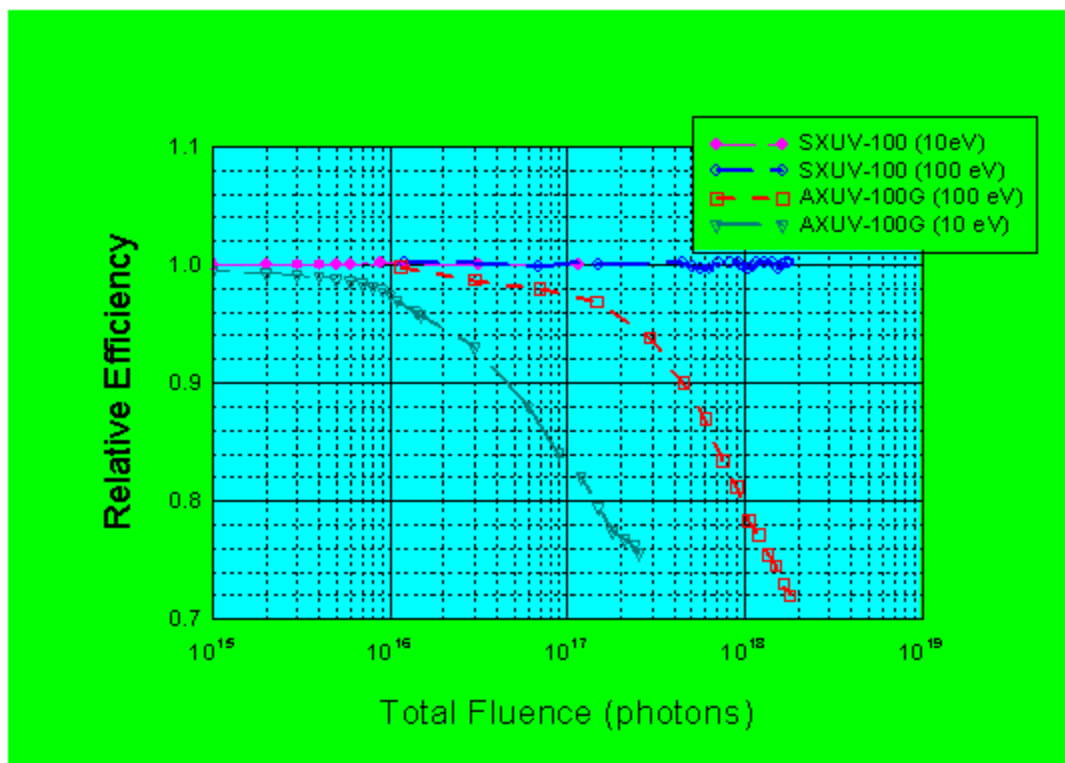
Fig. 3: Relative responsivity of SXUV and AXUV series photodiodes when exposed to 10 eV and 100 eV photons.
