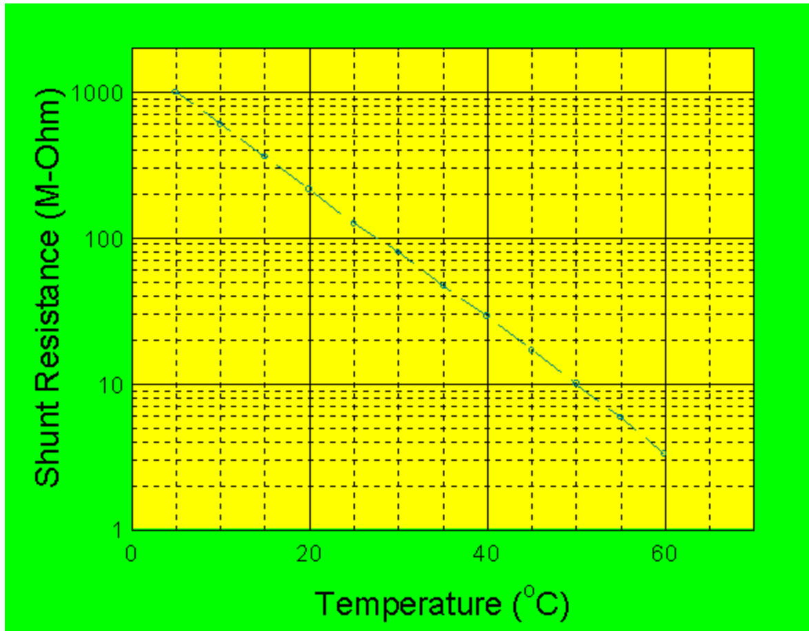
Fig. 2: Temperature dependence of Shunt Resistance of the SXUV-100 photodiode
