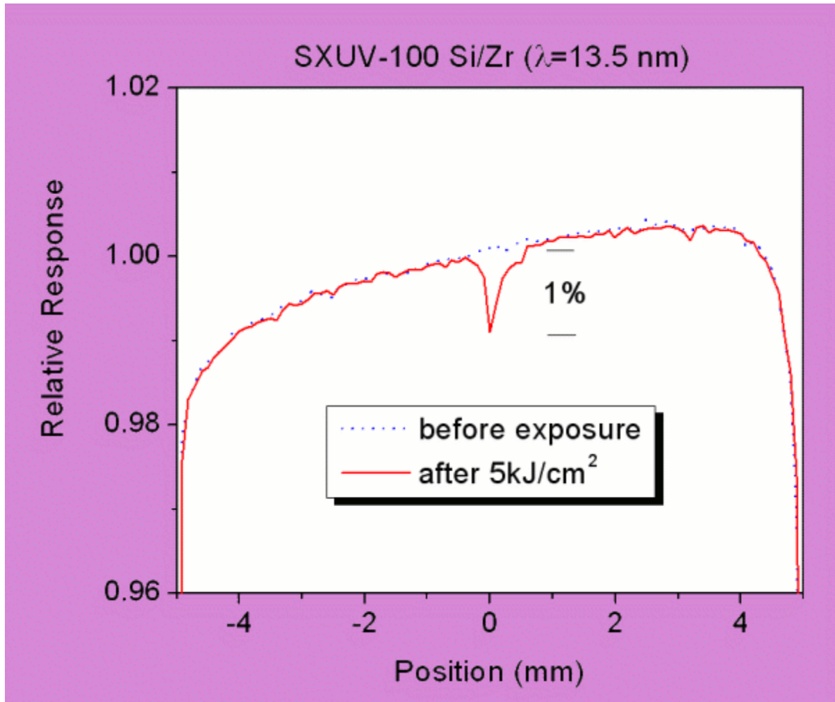
Fig. 5: Line scan of the SXUV-100 Si/Zr diode with 13.5 nm beam before and after exposure to 4 \times 10^{20} 60-110 eV photons
