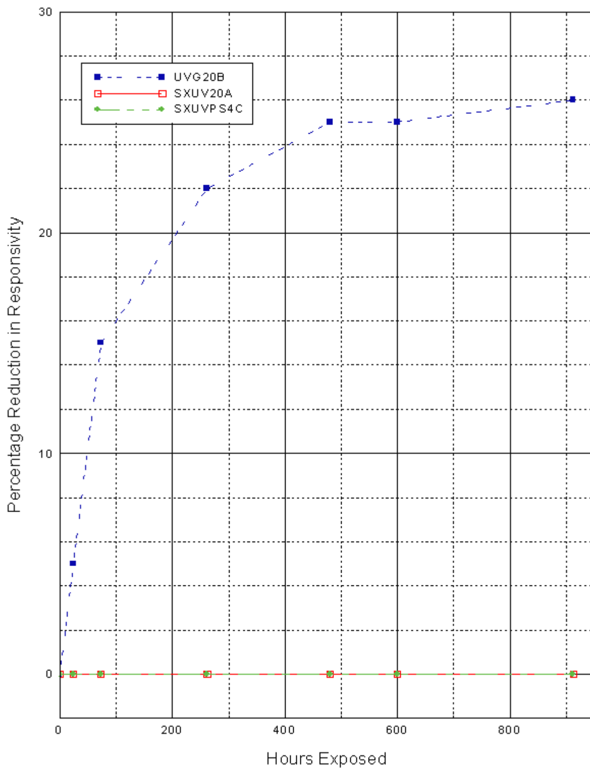
Fig. 5: Relative responsivity of SXUV and AXUV series photodiodes when exposed to 6.53 \text{ mW/cm}^2 185 nm lamp irradiation.
