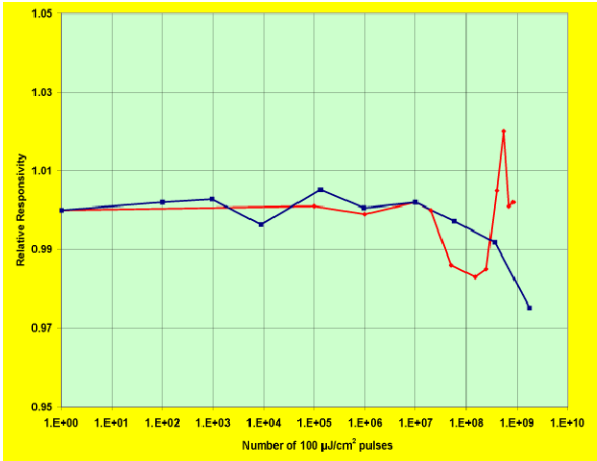
Fig. 2: Responsivity stability of SXUV series photodiodes after exposure to 193 and 157nm excimer laser: -193nm, -157nm
