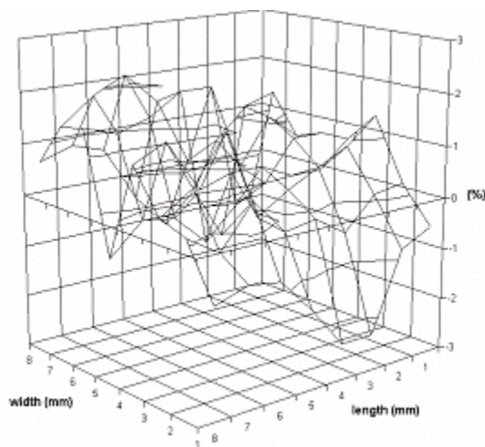
Fig. 1: Spatial responsivity uniformity of the SXUV-100 photodiode at 121.6 nm
