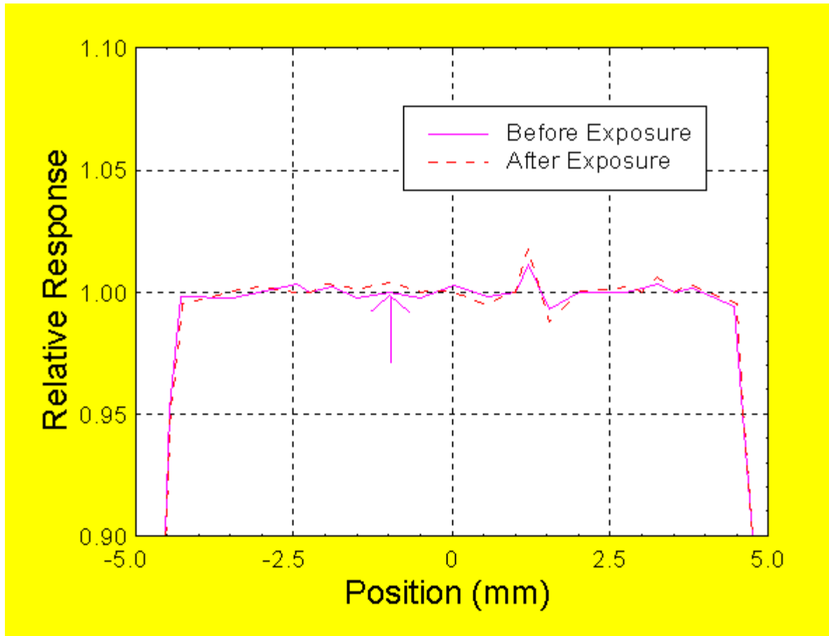
Fig. 4: Line scan of the SXUV-100 diode with 12.4 nm beam before and after exposure to 10^{22} photons/cm 2 100 eV photons
